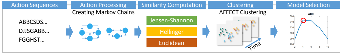
Figure 7.1: Overview of our clustering pipeline. Action sequences are extracted from log data and transformed into Markov Chains per session. Pairwise similarities between students are computed for every session. Clustering is performed using evolutionary clustering. Finally, the AICc criterion selects the best model.
