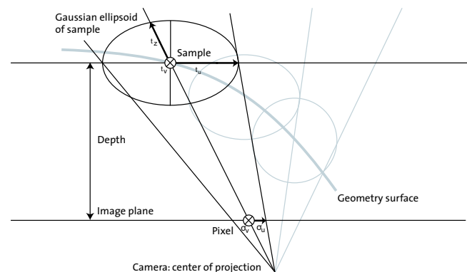
Fig. 6 Construction of a 3D Gaussian ellipsoid.
