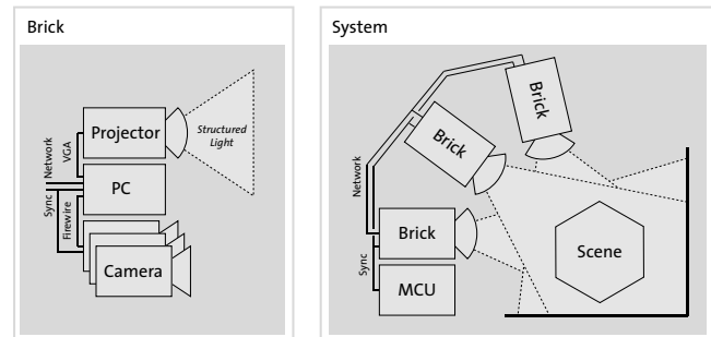
Fig. 3 Configuration of our 3D video prototype system.
