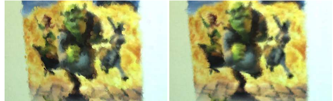
Fig. 9 Rendering using surfels (left) and our view-dependent uncertainty blending (right).
