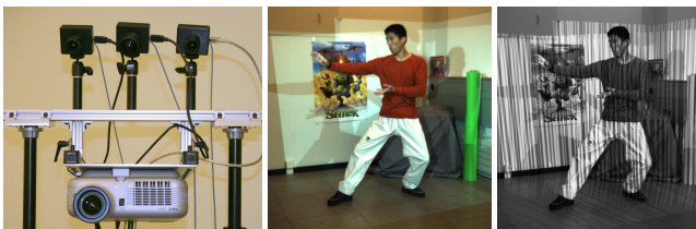
Fig. 2 3D video brick with cameras and projector (left), simultaneously acquiring textures (middle) and structured light patterns (right).
