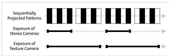
Fig. 4 Camera exposure with inverse pattern projection.
