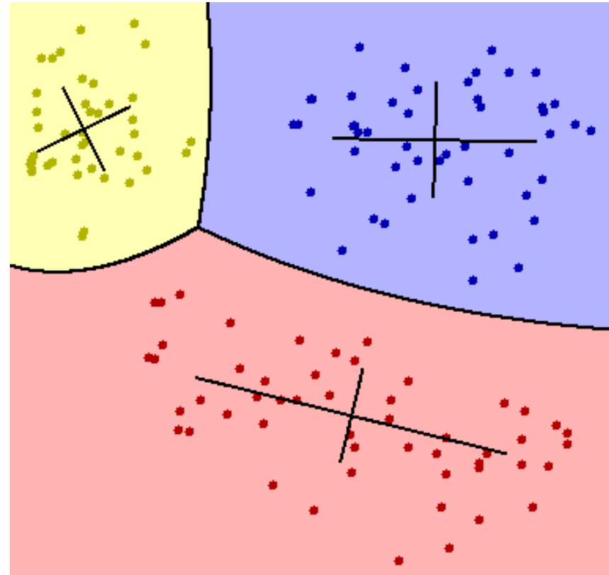
Figure: three Gaussian densities are fitted to the given data samples. The crosses denote the principal axes of the Gaussians.
