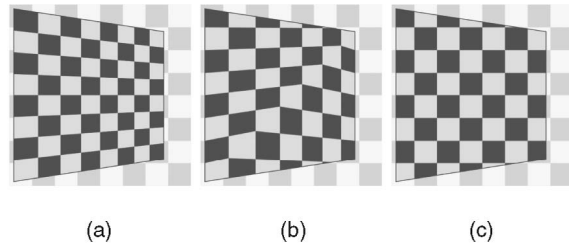
Fig. 4. Screen-space interpolation of texture coordinates. (a) The rasterizer interpolates vertex attributes in perspective space, which is typically used to map a 2D texture onto the faces of a 3D object. (b) Using the projected vertices of a primitive as texture coordinates to perform a lookup in a screen-space buffer yields incorrect results unless the primitive is parallel with the screen. (c) Computing the texture coordinates directly from the fragment window position or using projective texture mapping results in the desired screen-space lookup.
