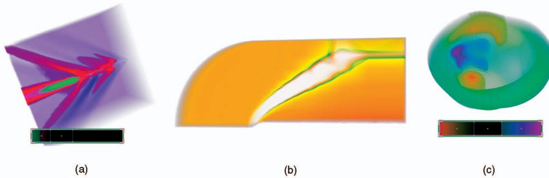
Fig. 1. Results of volume rendering the (a) fighter, (b) blunt fin, and (c) heart data sets with the HAVS algorithm.
