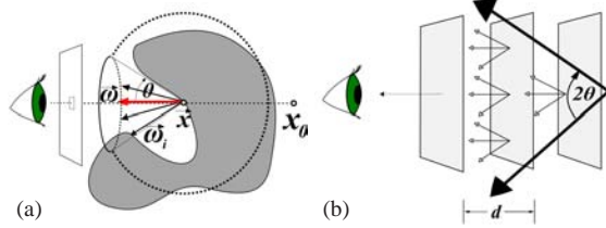
Figure 1: a) The geometric setup of the proposed direct occlusion shading model showing the conical subset of the sphere used to compute the occlusion. b) The setup used for the interactive computation of the occlusion factors.
