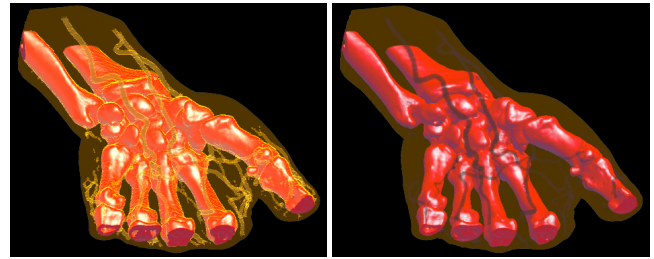
Figure 27: Detecting changes in compositing mode for each individual sample along a ray can be done exactly using two rendering buffers (left), or approximately using only a single buffer (right).
