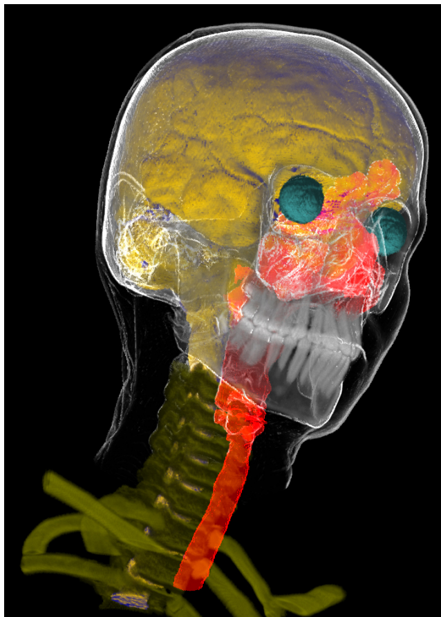
Figure 17: Segmented head and neck data set (256x256x333) with eight different enabled objects – brain: tone shading; skin: contour enhancement with clipping plane; eyes and spine: shaded DVR; skull, teeth, and vertebrae: unshaded DVR; trachea: MIP.
