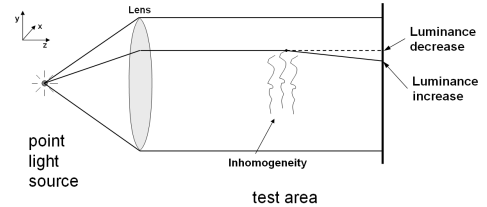
Figure 9: Simple Shadowgraph system diagram
