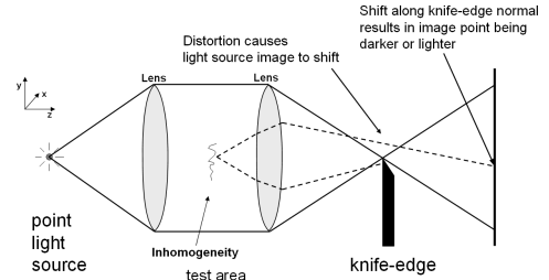
Figure 8: Simple Schlieren system diagram
