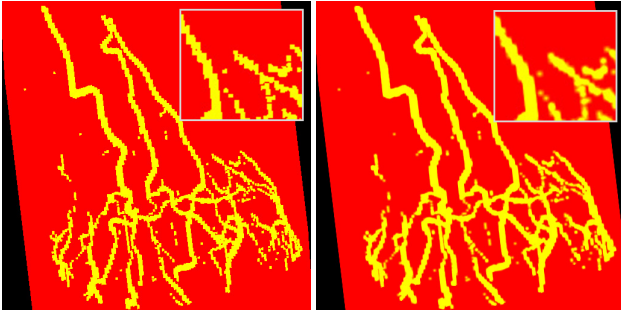
Figure 25: Selecting the transfer function on a per-fragment basis. In the left image, point-sampling of the object ID volume has been used, whereas in the right image procedural linear interpolation in the fragment shader achieves results of much better quality.
