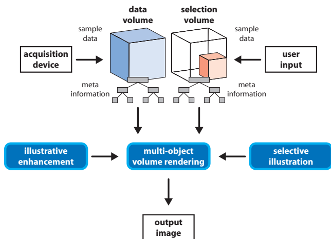
Figure 2: Conceptual overview of our direct volume illustration environment.
