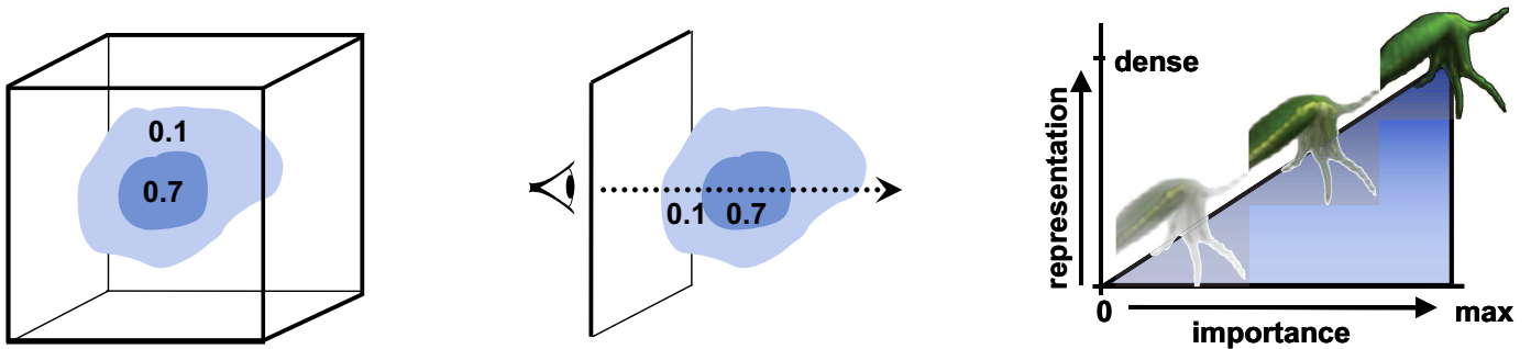
Fig. 2. Basic elements of importance-driven volume rendering: Volumetric features are classified by importance values (left). The volume is traversed in the importance compositing step (middle). Then levels of sparseness are chosen to enhance or suppress particular parts of the volume (right).
