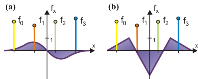
Figure 3: The first order (a) and second order (b) derivatives of the cubic B-spline filter for direct high-quality reconstruction of derivatives via convolution.
