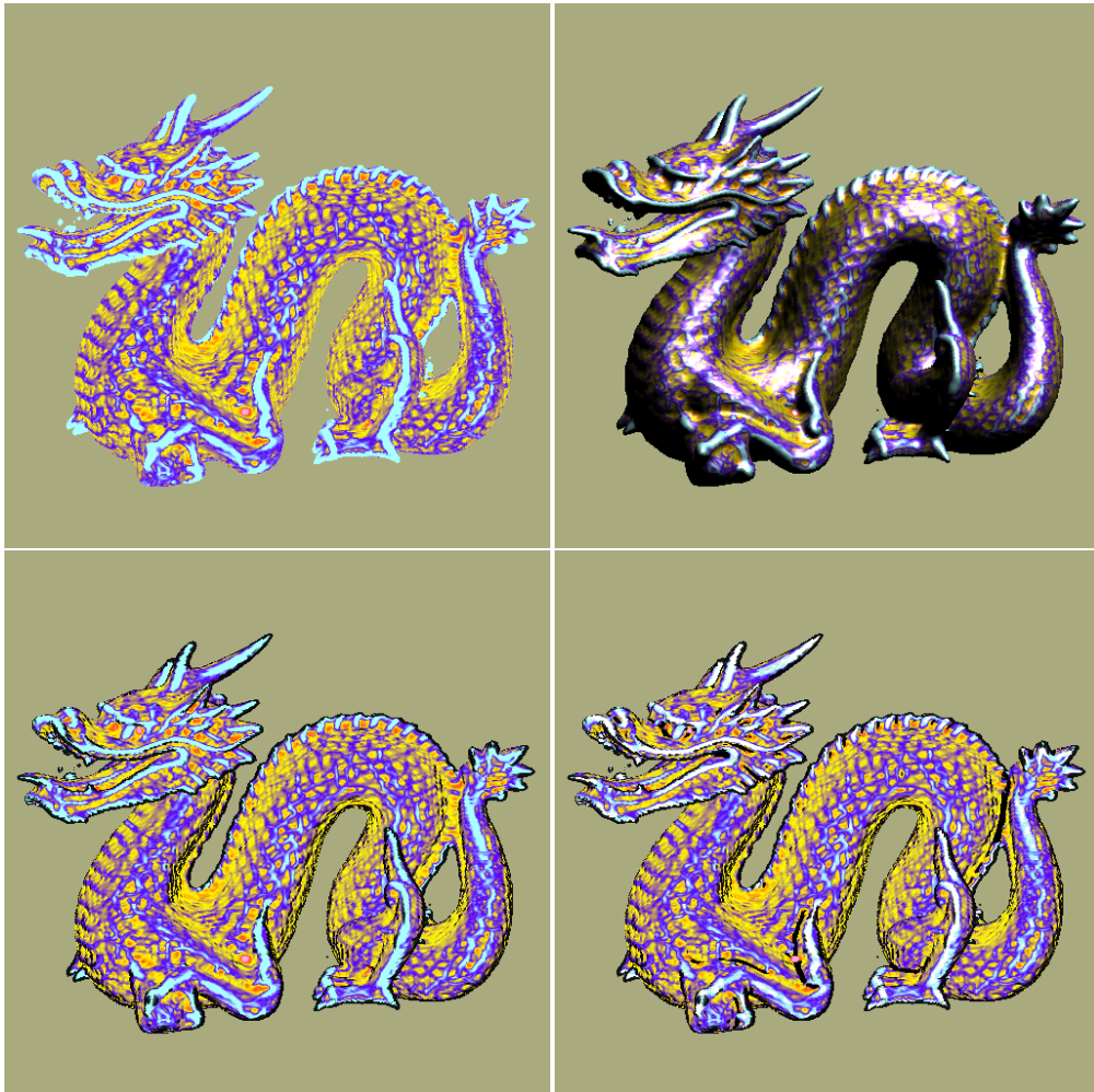
Figure 13: Dragon distance field (128x128x128) with colors from curvature magnitude (top, left); with Phong shading (top, right); with contours (bottom, left); with ridge and valley lines (bottom, right).
