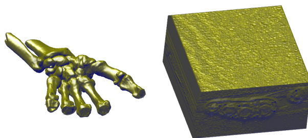
Figure 21: In order to render the bone structure shown on the left, many voxels need to be culled. The early z-test allows to avoid evaluating shading equations for culled voxels. If it is not employed, performance will correspond to shading all voxels as shown on the right.
