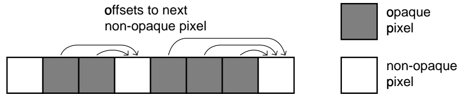
Figure 4.1: Offsets stored with opaque pixels in the intermediate image allow occluded voxels to be skipped efficiently.
